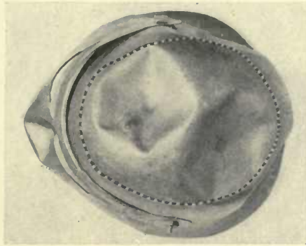
Fig. 169. Experimental helmet model No. 8. Result of test by pistol bullet at 800 f. s. Outline of head within helmet is shown by dotted line. This helmet bears marks of six testing bullets
