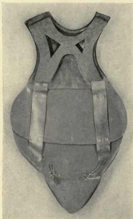
Fig. 197. Light body armor. Inner view of laminated breastplate. A heavy cushion of sponge rubber lines the uppermost plate
