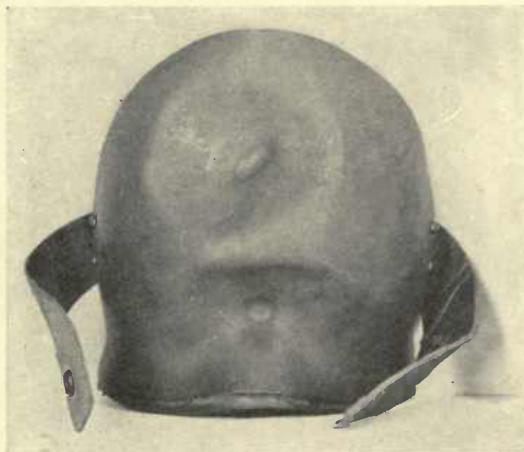
Fig. 188A. Result of test on foregoing face-guard, with pistol bullet at 850 f. s.
