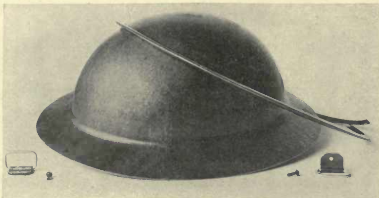
Fig. 146. Manufacture of British-American helmet. Helmet shell, metal rim, chin-strap loops and rivets ready to be put together
