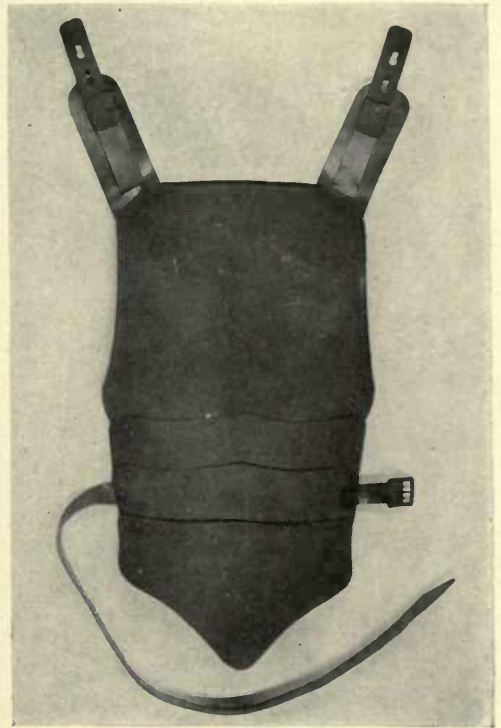
Fig. 198A. Laminated backplate of experimental model, 1918
