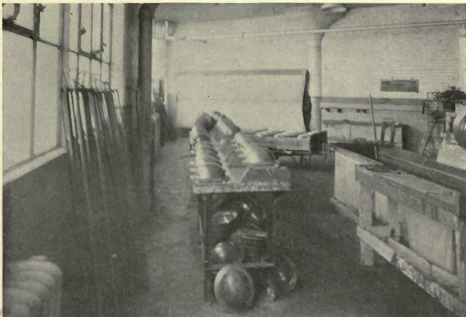
Fig. 152. British-American helmet. Assembling. The helmets are shown arranged in rows on metal racks, front and back, ready to be immersed in the paint trough shown in right of picture. (Ford Mfg. Co., Philadelphia)
