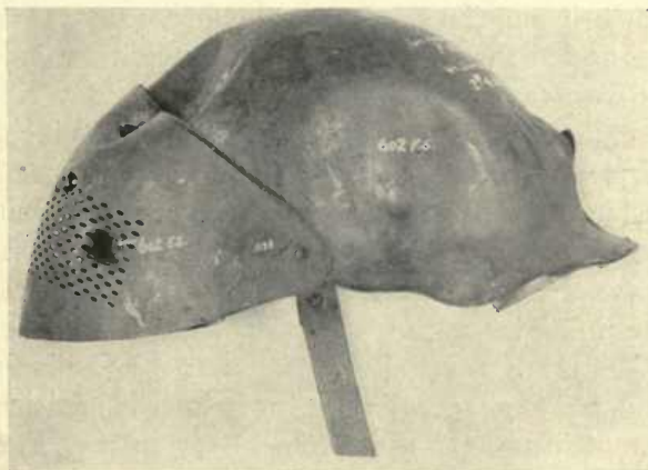
Fig. 116. Belgian helmet. Result of tests
