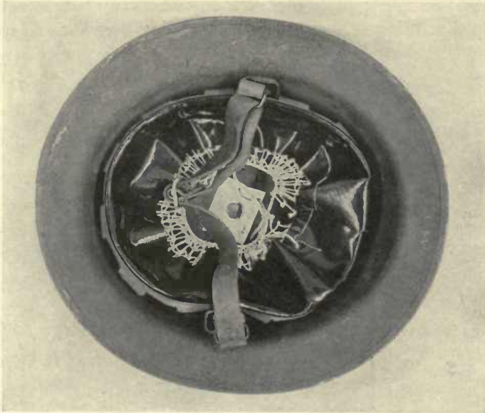
Fig. 87. British helmet viewed from below
